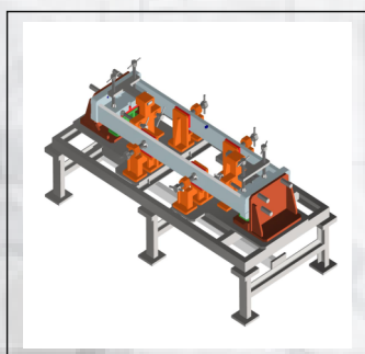
Welding Fixtures
