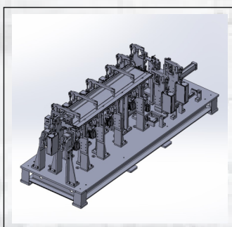
BIW Fixtures
