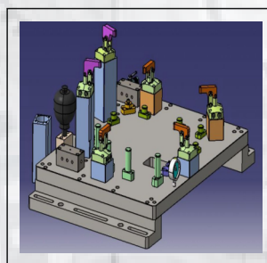
Hydraulic Fixtures
